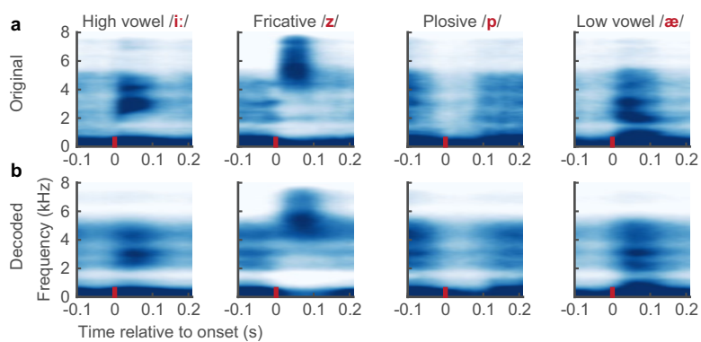
Extended Data Fig. 1 | Median original and decoded spectrograms. a, b , Median spectrograms, time-locked to the acoustic onset of phonemes from original ( a ) and decoded ( b ) audio (/i/, n = 112 ; /z/, n = 115 ; /p/,
